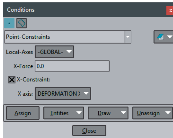
Conditions window in GiD Preprocessing
