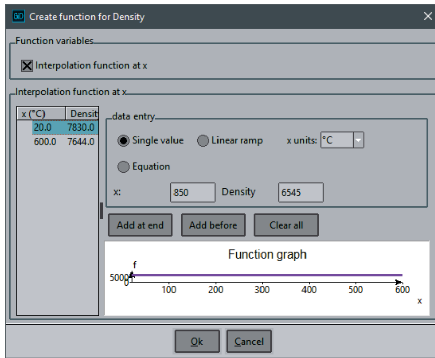
Interpolation function window
