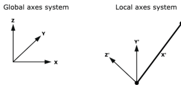
Local axes system X□Y□Z□ assigned on a line element
