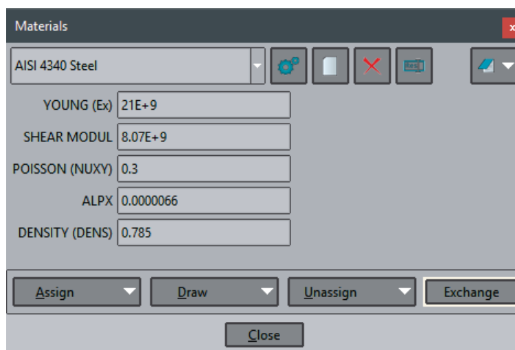
Materials window in GiD Preprocessing
