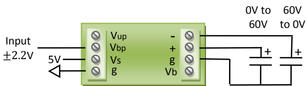
60 V Push-pull stack driver or bender driver
