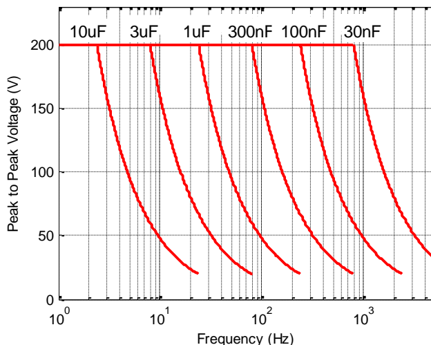
Figure 5. 100 V range power bandwidth
