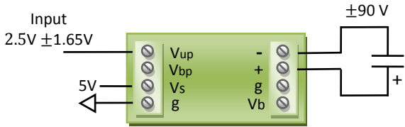
±90 V Piezo bender driver with unipolar input
